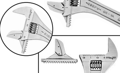
Reversible Jaw for Work on Bolts and Round Stock
